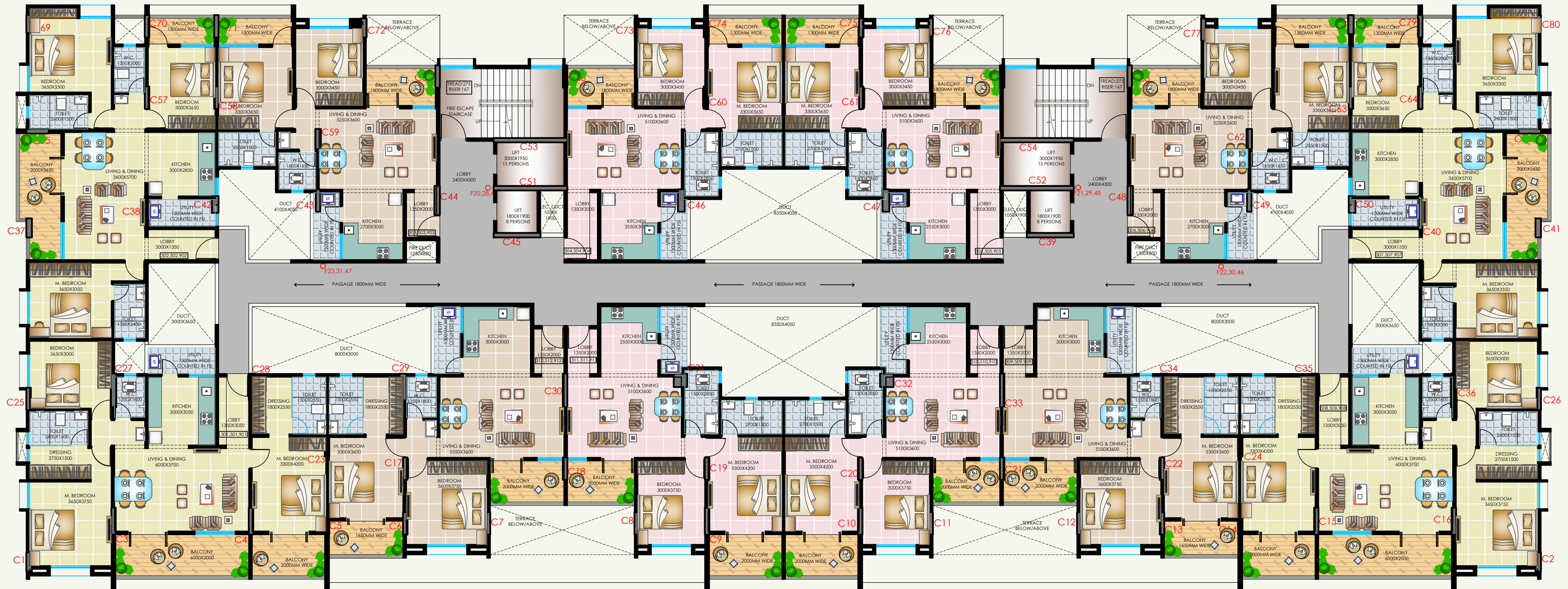
TYPICAL THIRD, FIFTH AND NINTH FLOOR PLAN
